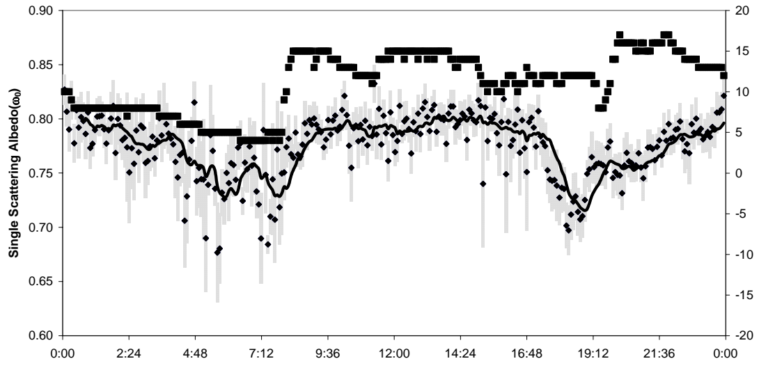
Fig. 11 Diurnal cycle of Single Scattering Albedo from PSAP and Nephelometer with error bars (light gray) and the number of data points from PSAP contributing to the average (squares).
