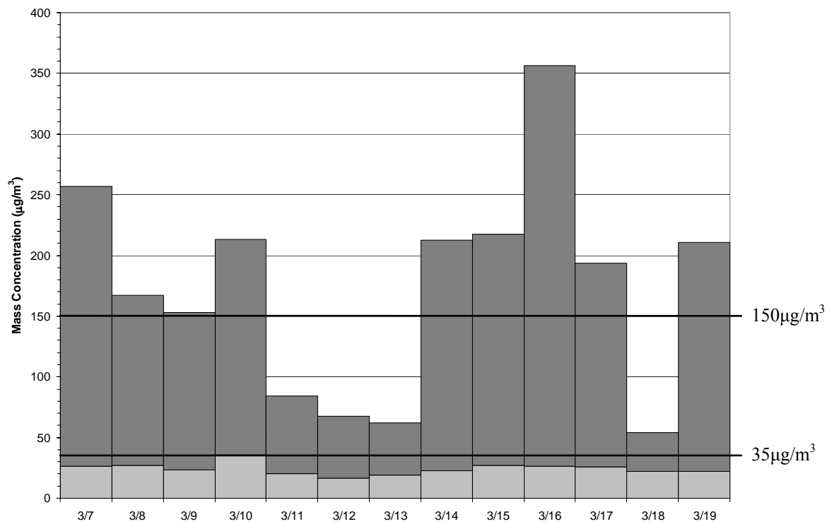
Fig. 2 Twenty-four hour averages of PM2.5 (light gray) and PM10 (total column) during the Intensive Observation Campaign compared to the US NAAQS 24-hour limit for particulate matter.
