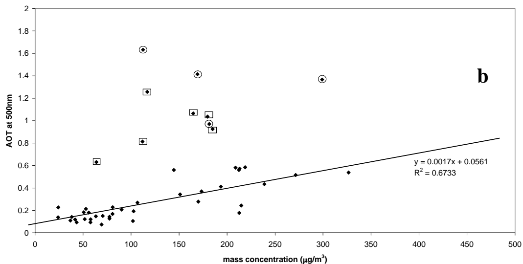
Fig. 5 a) Fine mode and b) PM10 concentrations versus AERONET AOT at 500nm. The marked points are not included in the correlation; circled points indicate lack of agreement from the SMR comparison in figure 3 while squared points indicate lack of AERONET size distribution data.
