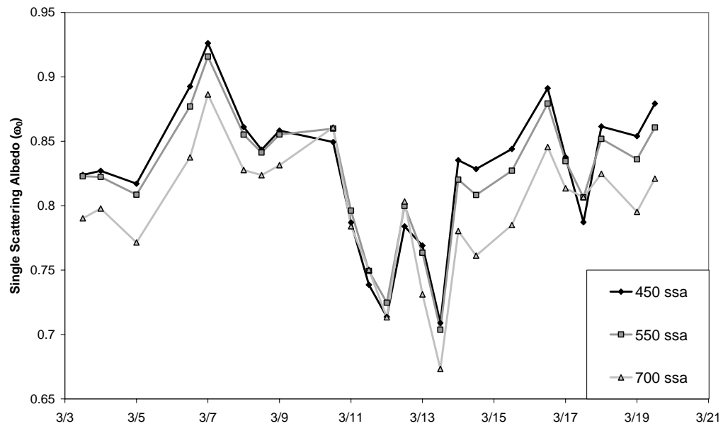
Fig. 9 Single Scattering Albedo ( \omega_0 ) from Optical Reflectance combined with the Nephelometer scattering coefficient at the three operating wavelengths: 450, 550, 700nm.
