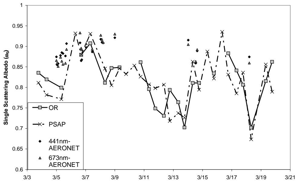
Fig. 10 Single Scattering Albedo from AERONET and a combination of the scattering coefficient from the Nephelometer at 550nm with Optical Reflectance and PSAP results.
