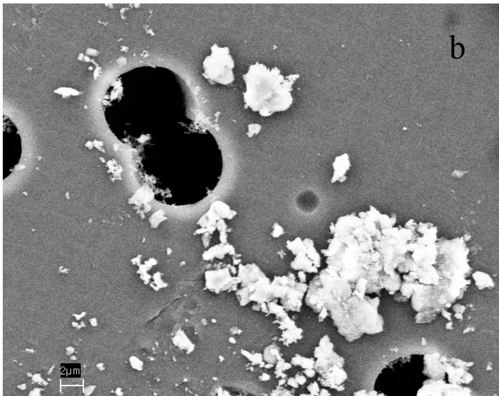
Fig. 7 Scanning Electron Microscope image of a) March 10, 2005 fine mode filter and b) March 12, 2005 coarse mode filter. The scale in figure a corresponds to 1\mu\text{m} and the scale in figure b corresponds to 2\mu\text{m} . The black circles shown are the filter pores whereas the particles are shown in white and gray tones.
