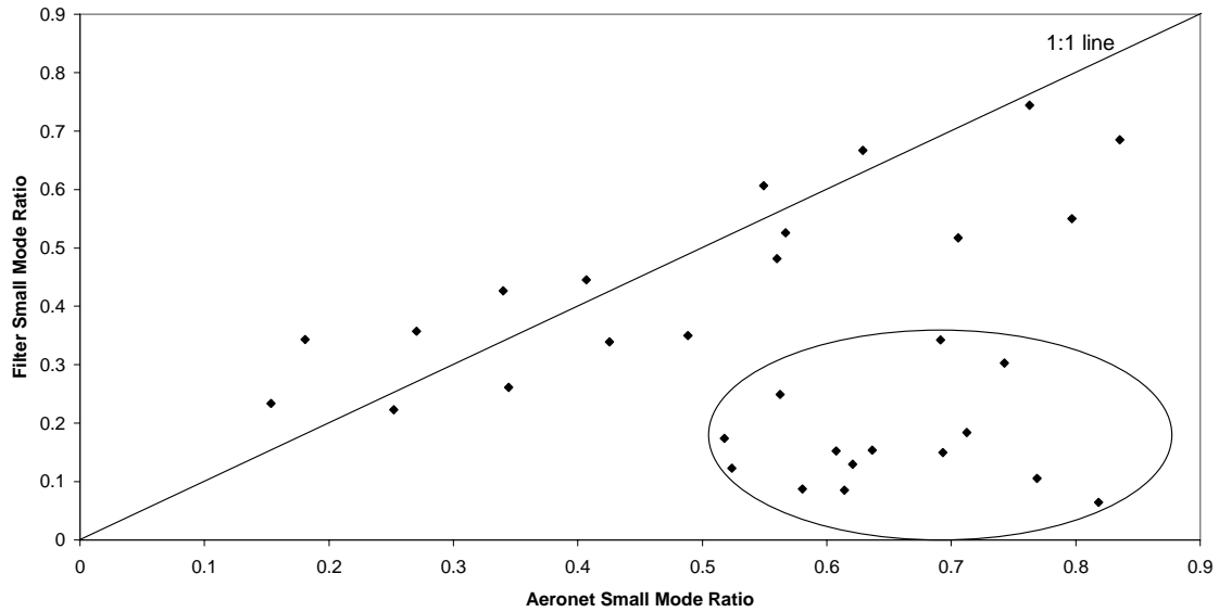
Fig. 3 Comparison between calculated AERONET Small Mode Ratio versus the measured filter Small Mode Ratio for available data from January 13-May 24, 2005. AERONET results were calculated from the average of almucantar inversions performed throughout the day, whereas the filter data was sampled during the daylight hours. The 1:1 line is shown in the plot to indicate cases of good agreement between both results. Cases of poorer agreement are circled.
