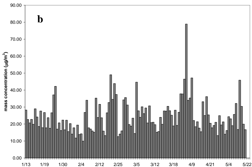
Fig. 1 Twelve-hour Mass Concentration of a) coarse mode particles with aerodynamic diameter 2.5\mu\text{m} < d < 10\mu\text{m} , and b) fine mode particles with d < 2.5\mu\text{m} for the period between January 13-May 24, 2005 in Xianghe, China.
