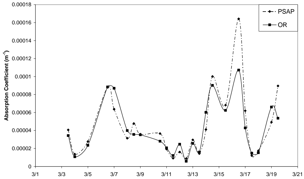
Fig. 8 Comparison of absorption coefficient from the Optical Reflectance (OR) technique applied to the Nuclepore filters and the corresponding average PSAP results during the IOP.
