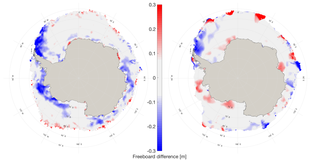
Figure 10: Snow freeboard differences showing (left) CryoSat-2 October 2011-2017 average minus ICESat spring 2003-2007 average and (right) ICESat spring 2006 average minus ICESat spring 2003-2007 average. 2006 is included as an example year to highlight the interannual variability in the freeboard distribution.
