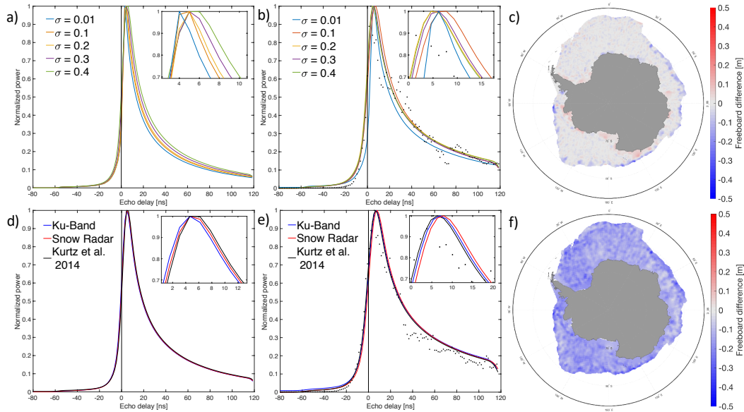
Figure 6: A sensitivity study of two initial guess parameters: the standard deviation of surface height and the total backscatter. (a) modeled waveform (before fitting) varying the initial guess value of \sigma between 0.01 (very smooth surface) and 0.4 (rough surface). (b) waveforms fit to CryoSat-2 data varying the initial guess value of \sigma between 0.01 and 0.4. (c) October 2016 average freeboard difference: \sigma = 0.35 as the initial guess – \sigma = 0.15 as the initial guess. (d) as in (a) using three different backscatter parameterizations taken from the OIB Ku-Band radar profile, Snow Radar profile, and Kurtz et al. 2014. (e) as in (b) with the three different backscatter parameterizations. (f) as in (c) showing Kurtz et al. 2014 backscatter as the initial guess – Ku-Band backscatter as the initial guess. Inlaid plots are zoomed in on the waveform peaks. The methodology for freeboard calculations is explained in later sections of the paper.
