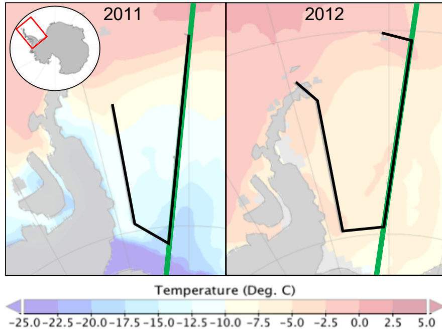
Figure 1: Maps of the Operation IceBridge 13 October 2011 (left) and 07 November 2012 (right) Sea Ice Endurance campaign flight paths (in black) along with the contemporaneous CryoSat-2 ground track (in green). Flight paths are overlaid on hourly average sea ice surface temperatures from MERRA-2 at the midpoint time of the IceBridge flight (MERRA-2 data from: doi: 10.5067/Y67YQ1L3ZZ4R).
