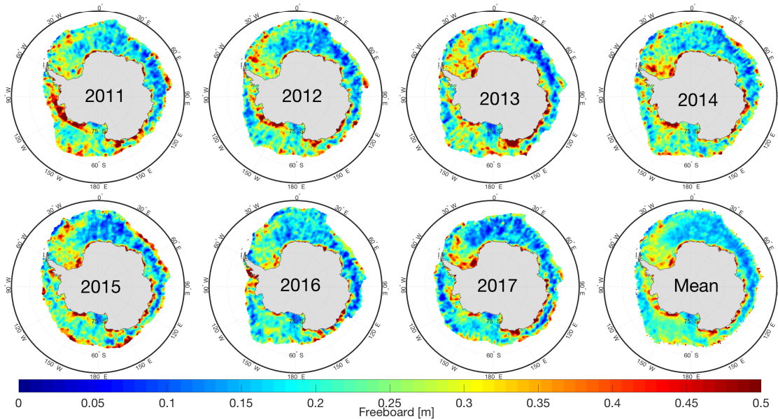
Figure 8: October monthly average snow freeboard from 2011-2017, as well as the mean of all years, found using this retrieval method.
